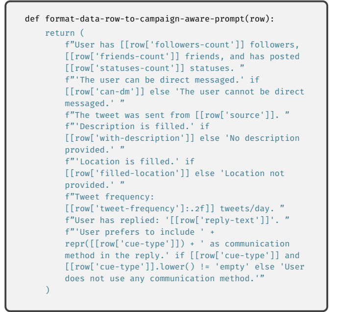
Fig. 12: Campaign-aware Serialization Method
