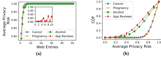
Figure 2: Risk prediction results of user Web entries. Here, (2a) average privacy risk with the increasing number of Web entries and (2b) Average privacy risk per user.
