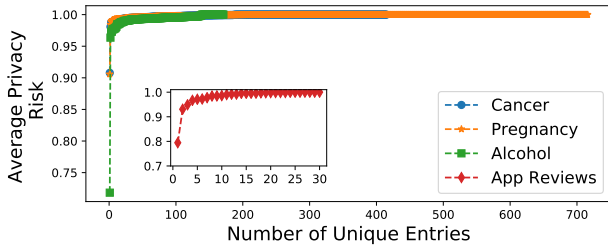
Figure 4: Risk prediction results of unique data sequences. X-axis is the number of unique sequences, while Y-axis is the average of risk entries against each sequence
