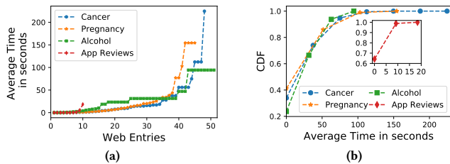
Figure 8: Results of average time against Web entries. Here, (8a) average time in seconds in the increasing order of Web entries; and (8b) CDF average time per user.
